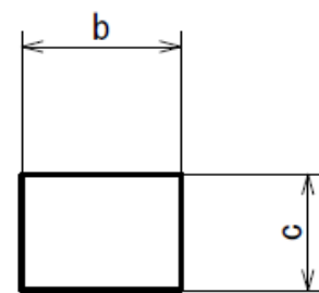
Terminal cross section (Ni/Pd/Au plating)
