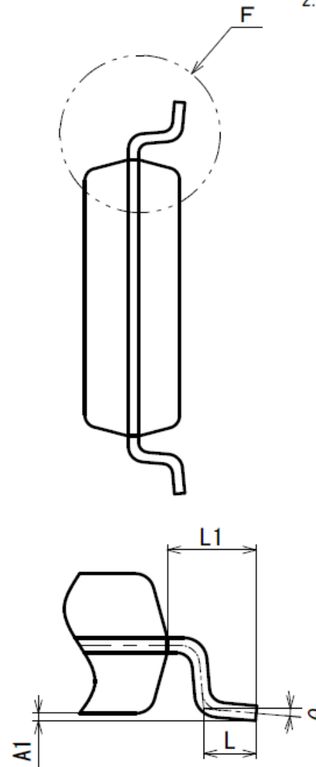
Terminal cross section (Ni/Pd/Au plating)
